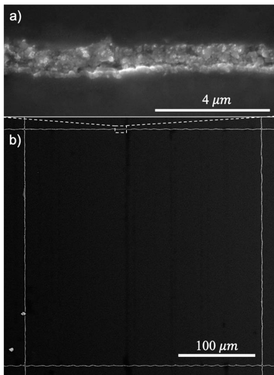
Fig.4 SEM images of the plated copper line (s: (a) narrowest linewidth of 804 nm), (b) copper grid with 1 \mu\text{m} linewidth and 300 \mu\text{m} spacing.
